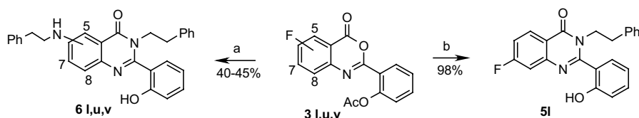
Scheme 2. Reagents and conditions: (a) \text{PhCH}_2\text{CH}_2\text{NH}_2 (2 equiv), 200 °C, 4 h; (b) \text{PhCH}_2\text{CH}_2\text{NH}_2 (2 equiv), DMF, microwave irradiation, 240 °C, 10 min. Compounds 3l : 7-F; 3u : 8-F; 3v : 5-F; 6l : 7-NHCH 2 CH 2 Ph; 6u : 8-NHCH 2 CH 2 Ph; 6v : 5-NHCH 2 CH 2 Ph.
