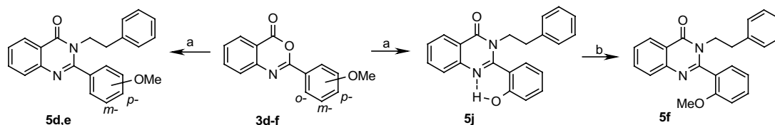
Scheme 4. Reagents and conditions: (a) \text{PhCH}_2\text{CH}_2\text{NH}_2 (2 equiv), 200^\circ\text{C} , 3 h; (b) MeI, \text{K}_2\text{CO}_3 , THF, \Delta , 24 h. Compounds 3 , 5 : d m -OMe; e p -OMe; f o -OMe.
