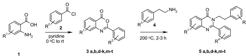
Scheme 1. Compounds 3 , 5 : \text{R}^2 = \text{R}^4 if \text{R}^2 \neq \text{OAc} or 2-OMe; \text{R}^4 = \text{OH} if \text{R}^2 = \text{OAc} or 2-OMe. For other substituents, see Tables 1 and 2 .
